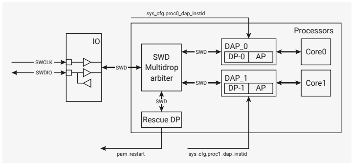
Figure 10. RP2040 Debugging
